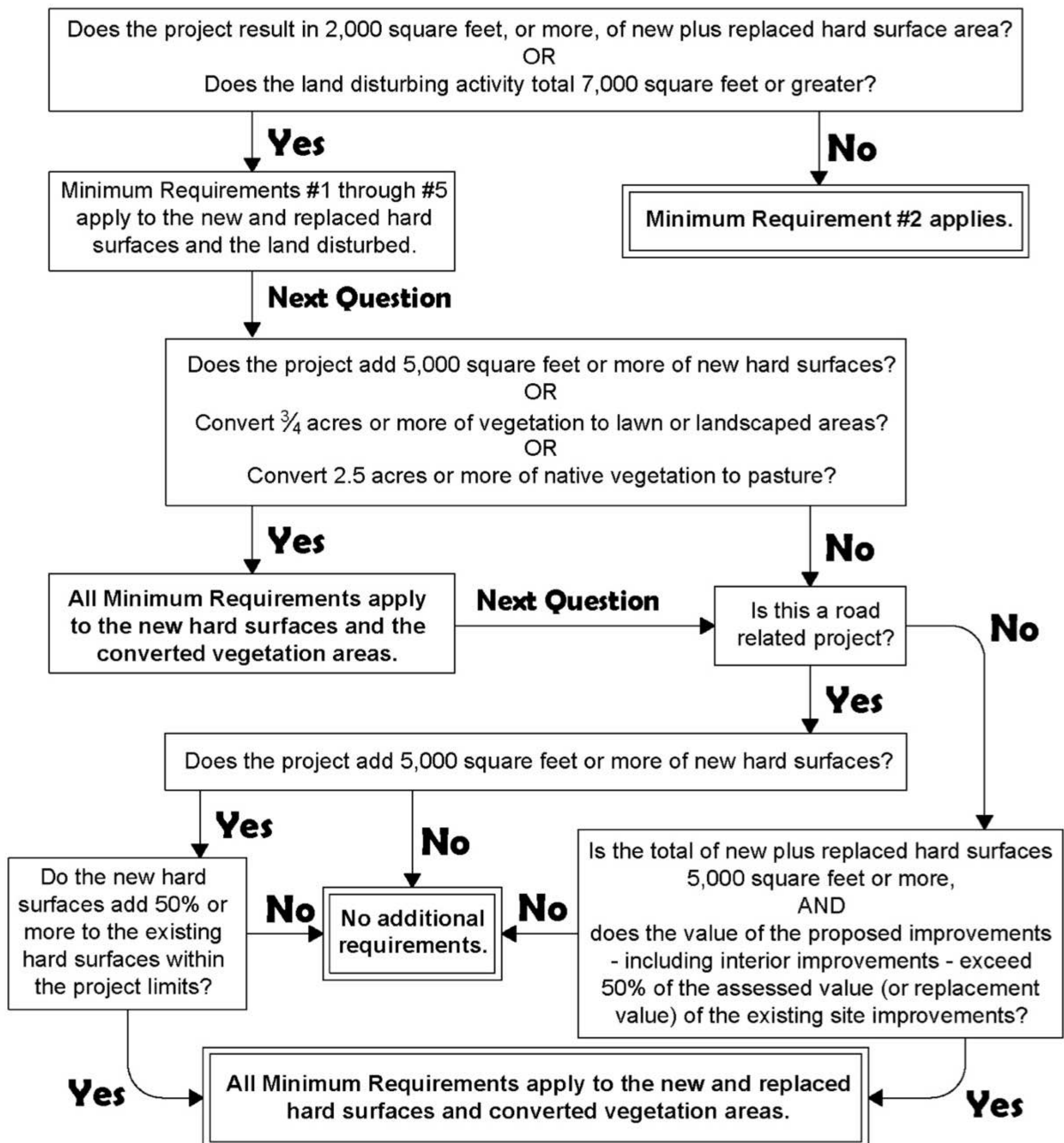
Figure II-2.4.2: Flow Chart for Determining Requirements for Redevelopment
