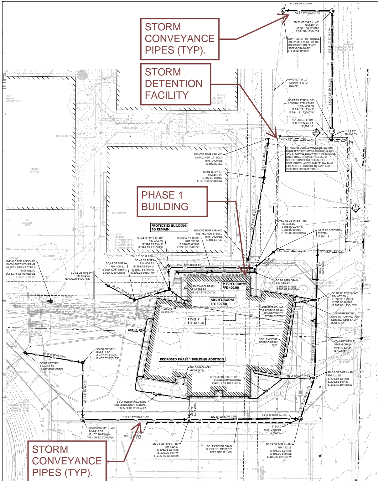
EXHIBIT A - SITE PLAN MUKILTEO ELEMENTARY SCHOOL - PHASE 1
