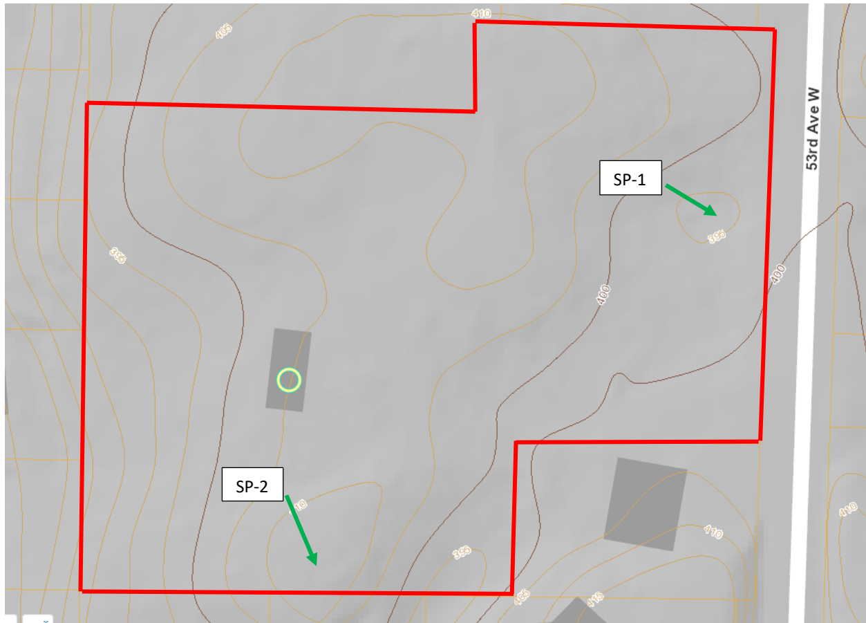
Figure 1—Wetland soil pits examined by Ecology at 9110 53 rd Ave W in the City of Mukilteo
